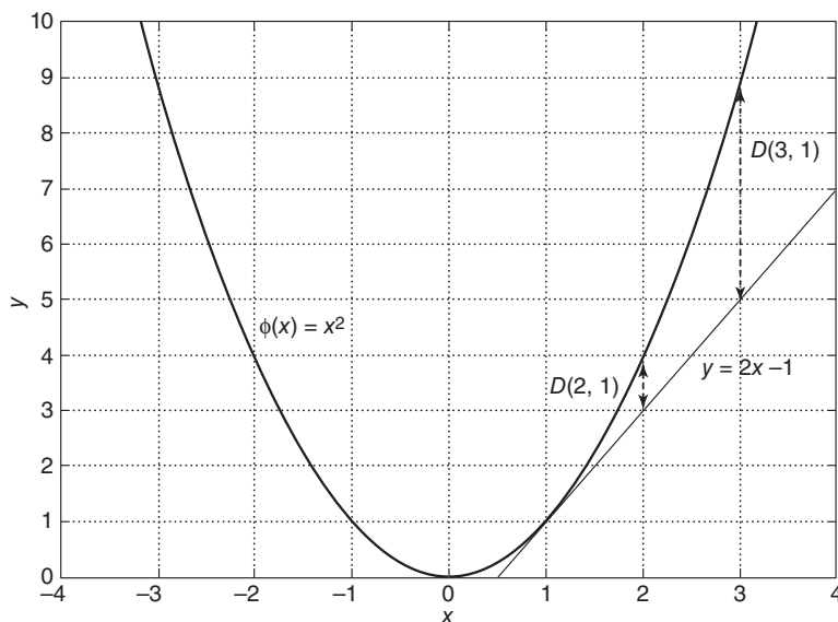
Figure 2.20. Illustration of Bregman divergence.
