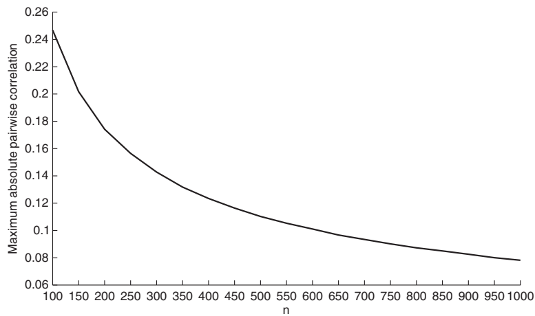
(a) Plot of maximum absolute pairwise correlation between 10 random vectors.
