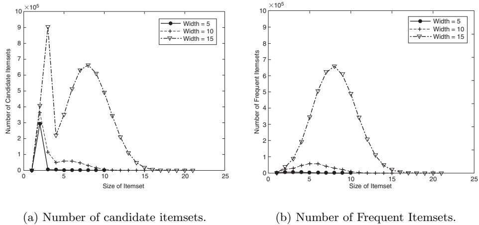
Figure 4.14. Effect of average transaction width on the number of candidate and frequent itemsets obtained from a synthetic data set.
