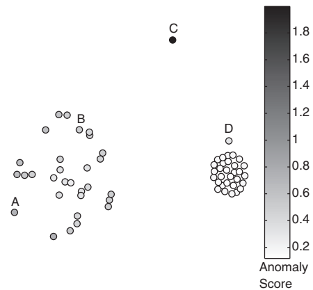
Figure 9.7. Anomaly score based on the distance to the fifth nearest neighbor, when there are clusters of varying densities.
