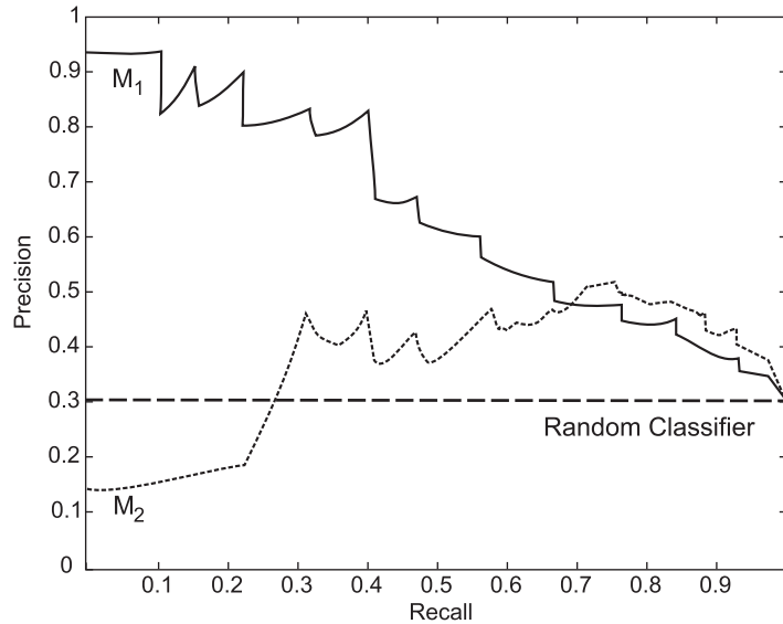
Figure 6.55. PR curves for two different classifiers.
