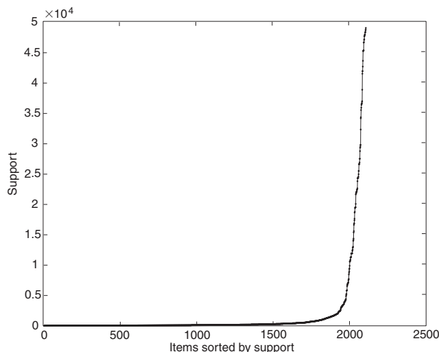
Figure 4.30. Support distribution of items in the census data set.
