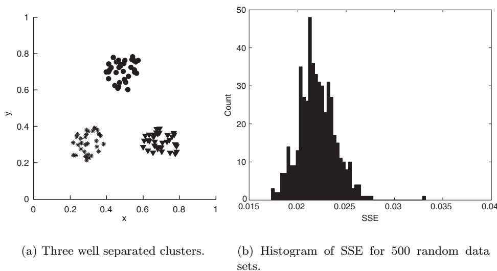
Figure 10.11. Using randomization to evaluate the p-value for a clustering.
