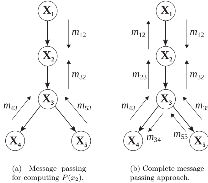
Figure 6.17. Illustration of message passing in the sum-product algorithm.
