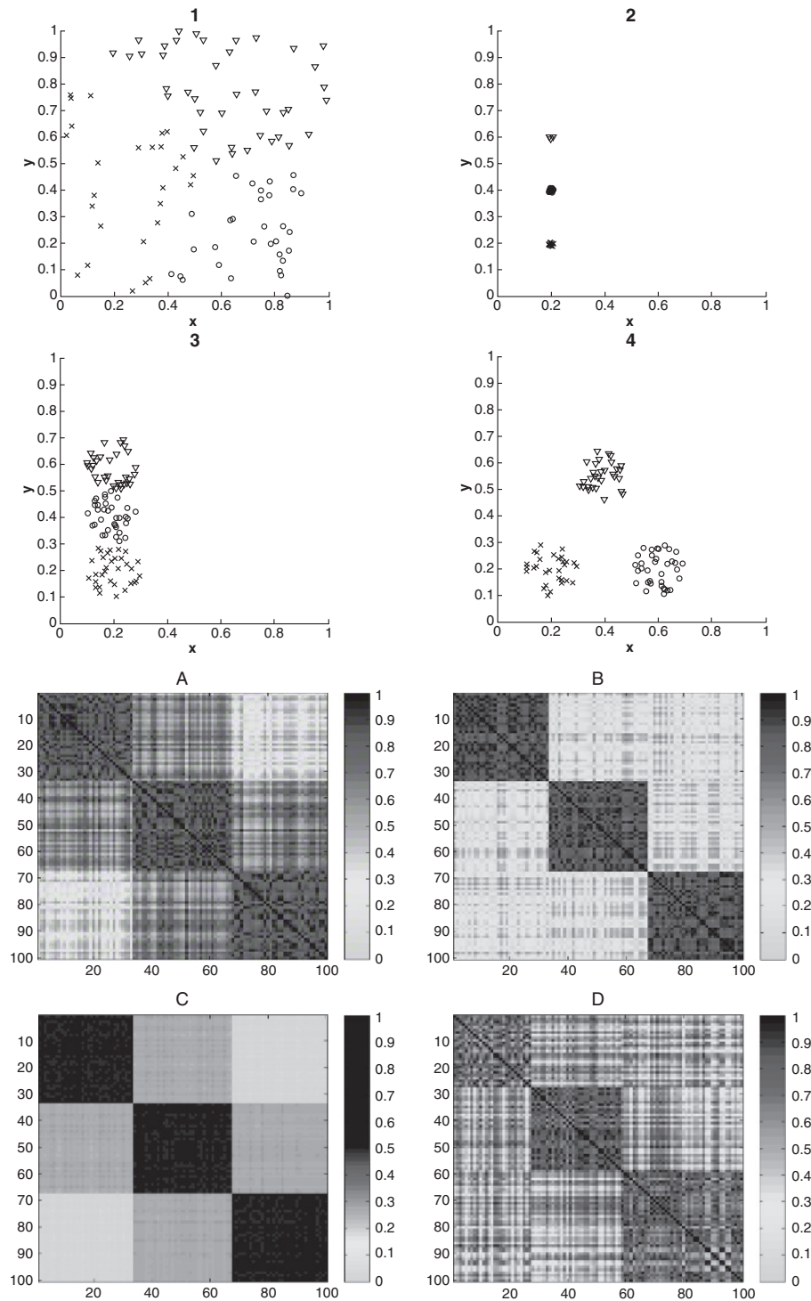
Figure 5.41. Points and similarity matrices for Exercise 37.
