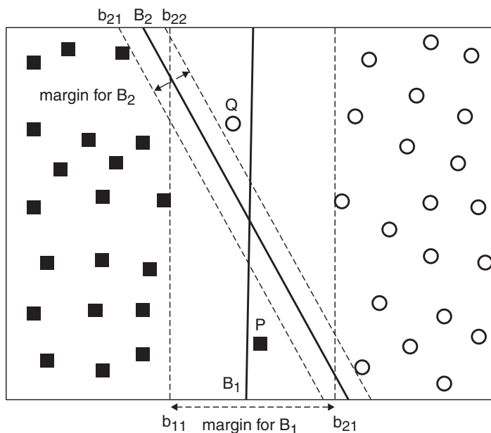
Figure 6.35. Decision boundary of SVM for the non-separable case.
