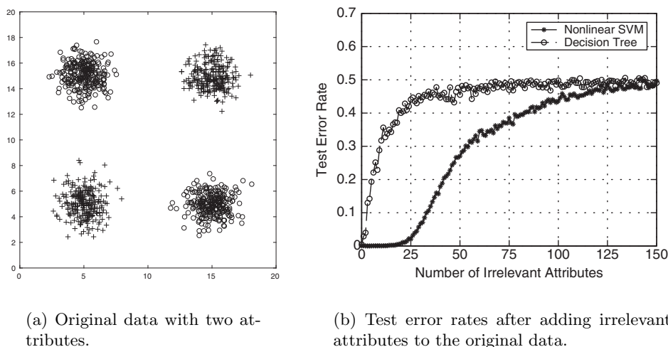
Figure 6.41. Comparing the effect of adding irrelevant attributes on the performance of nonlinear SVMs and decision trees.
