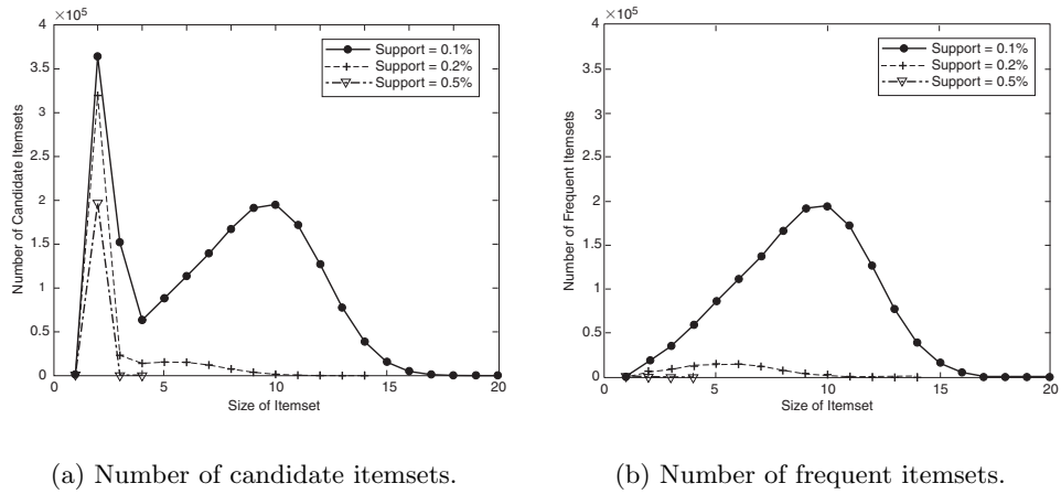
Figure 4.13. Effect of support threshold on the number of candidate and frequent itemsets obtained from a benchmark data set.
