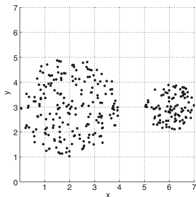
Figure 8.10. Grid-based density.
