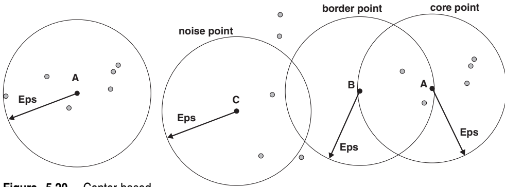
Figure 5.20. Center-based density.
