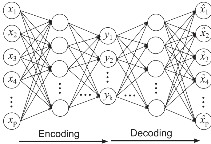
Figure 9.12. A basic architecture of the autoencoder.
